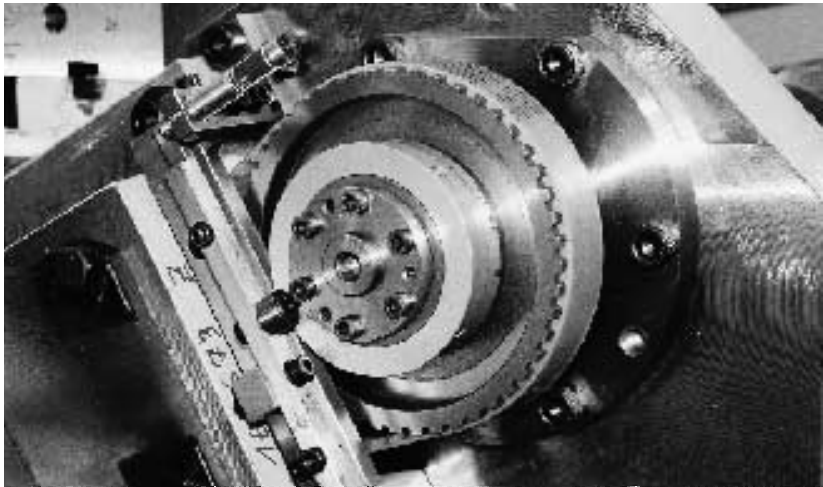
DMK/L coupling on a work spindle drive
