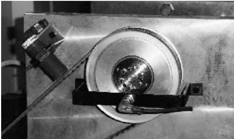
DMK/L 30 in a camshaft machining tool
